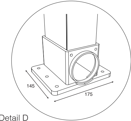
Detail D
