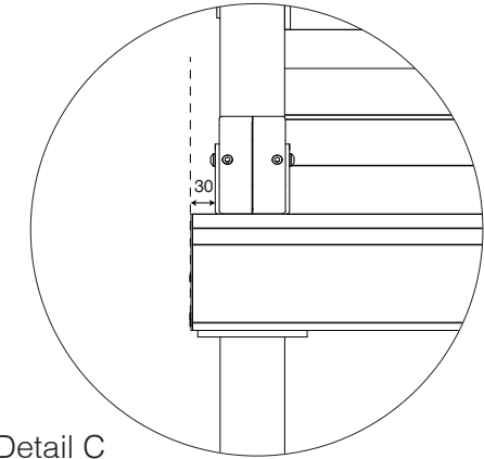
Detail C
