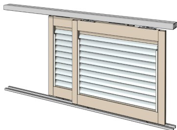
BOTTOM ROLLING SHUTTERS HAVE ALL THE WEIGHT ON THE BOTTOM TRACK
