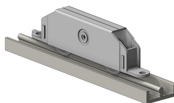
BOTTOM ROLLING SLIDER MECHANISMS
