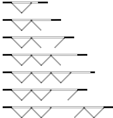
BIFOLDING CONFIGURATIONS
