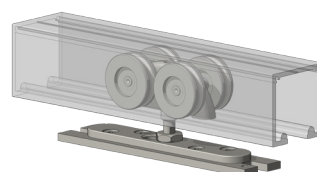
TOP HUNG SLIDER MECHANISMS
